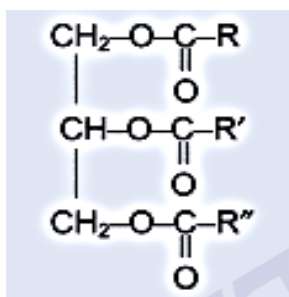
Figure 2.3: Structure of Vegetable Oil (Triglyceride) [1, 13]
