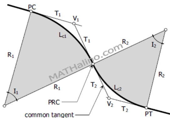
Figure 2.4: Layout of a reverse curve with parallel tangents (www.mathalino.com)
