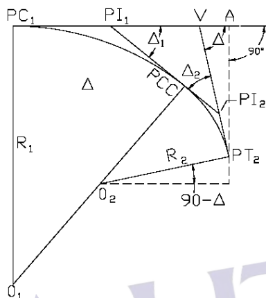
Figure 2.3: Layout of a compound curve (Garber & Hoel, 2009)
