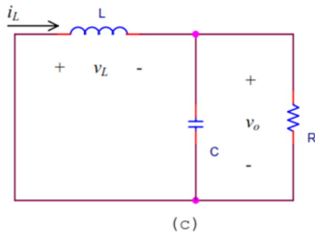
Figure 3: Buck converter during switch ON and OFF
