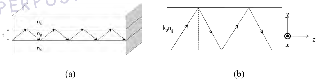
Figure 2.4 Planar slab optical waveguide structure and guiding layer
