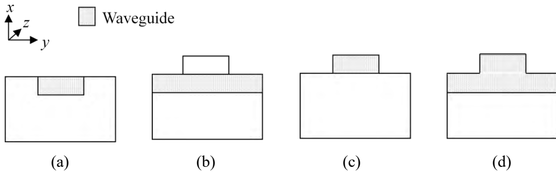
Figure 2.3 -x and -y view for the most common geometries for channel waveguide
