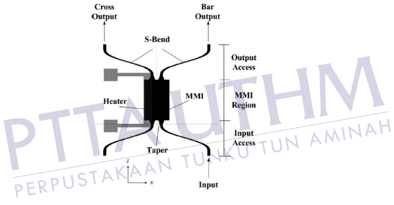
Figure 2.7 Schematic diagram of the MMI based optical switch (Wang et al. , 2006)
