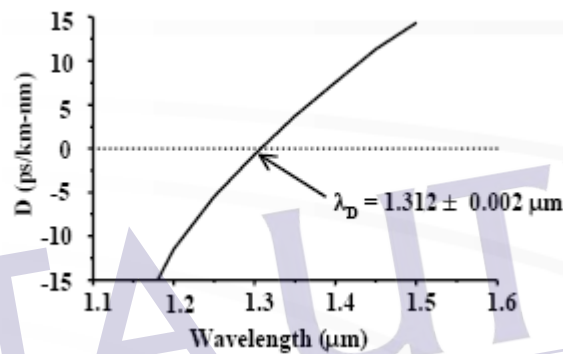
Figure 2.3: Variation of the dispersion parameter D with wavelength for a standard monomode fibre showing that zero dispersion occurs at \lambda \approx 1.3\mu\text{m} (Li T., 1985).
