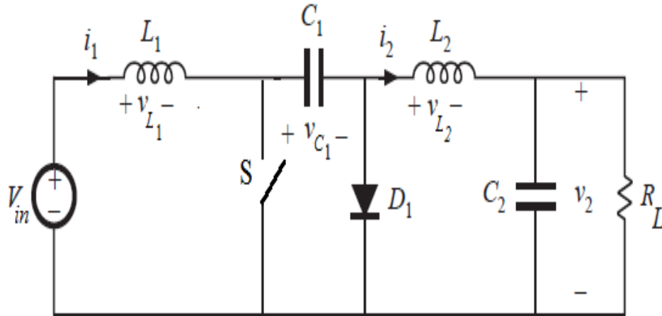
Figure 2.1: Cuk converter circuit
