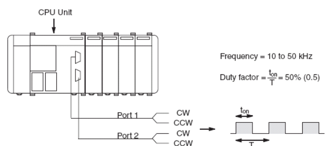
Figure 1 : Setting of rotation Direction of Stepper Motor
