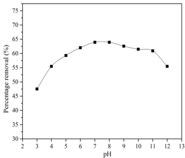
Fig. 3 Effect of pH on adsorption of colour
