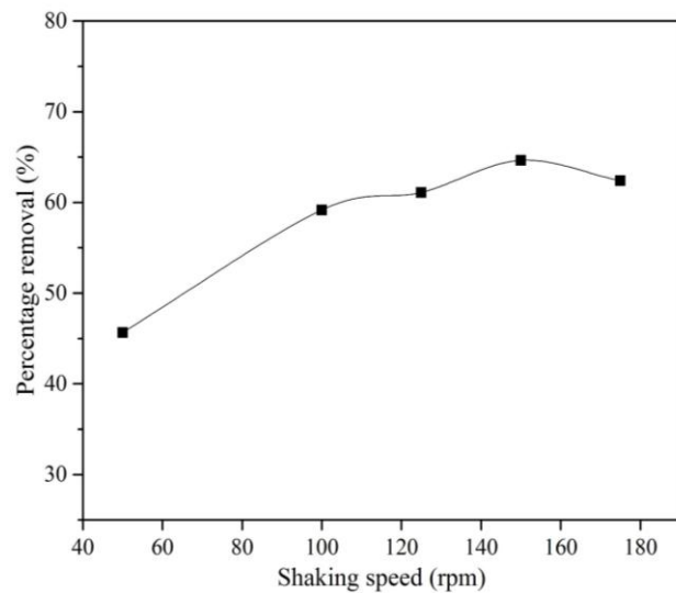
Fig. 4 Effect of shaking speed on adsorption of colour
