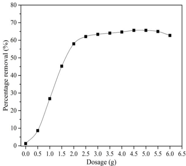
Fig. 2 Effect of chitosan bead dosage on adsorption of colour
