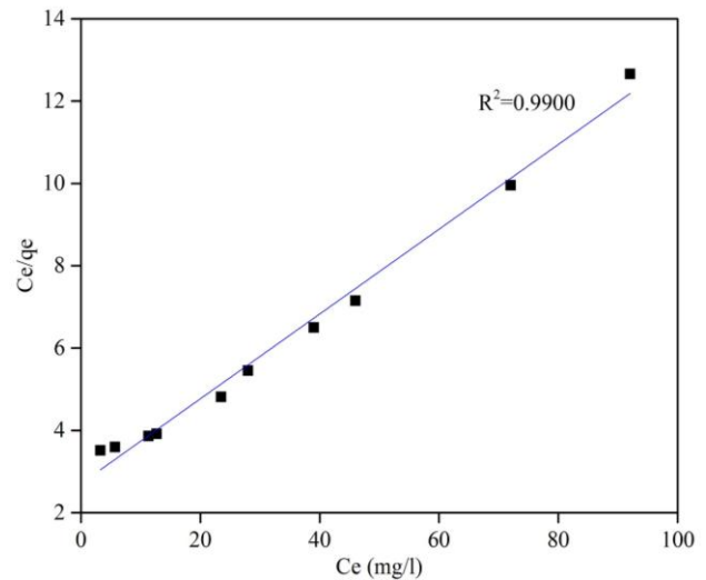
Fig. 6 Langmuir isotherm for adsorption of colour onto chitosan beads
