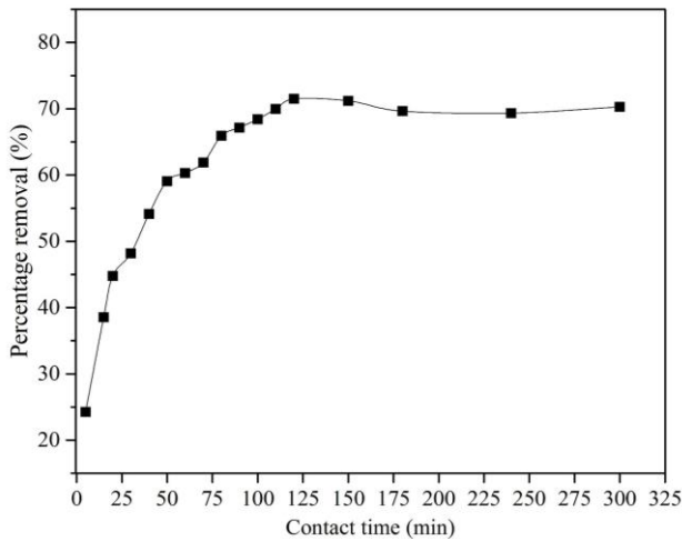
Fig. 5 Effect of contact time on adsorption of colour
