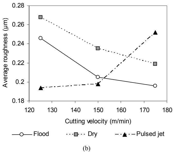
Fig. 2 Effect of cutting velocity on (a) flank wear and (b) surface roughness in slot milling test
