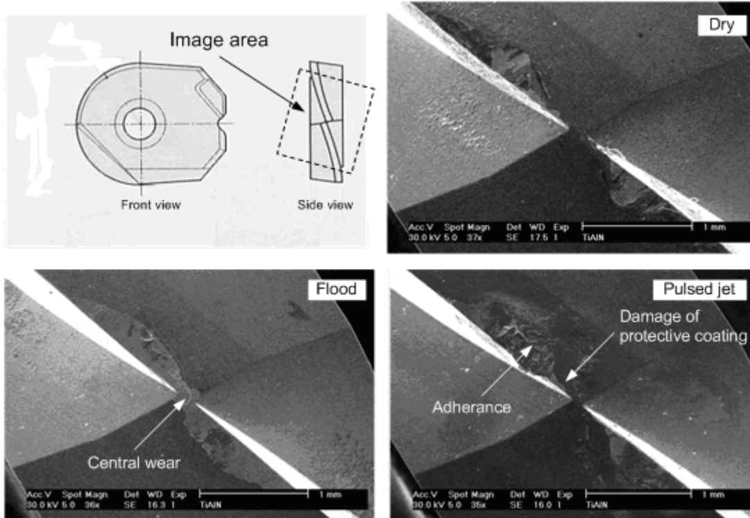
Fig. 8 Tools wear images when cutting in dry, flood and pulsed jet mode
