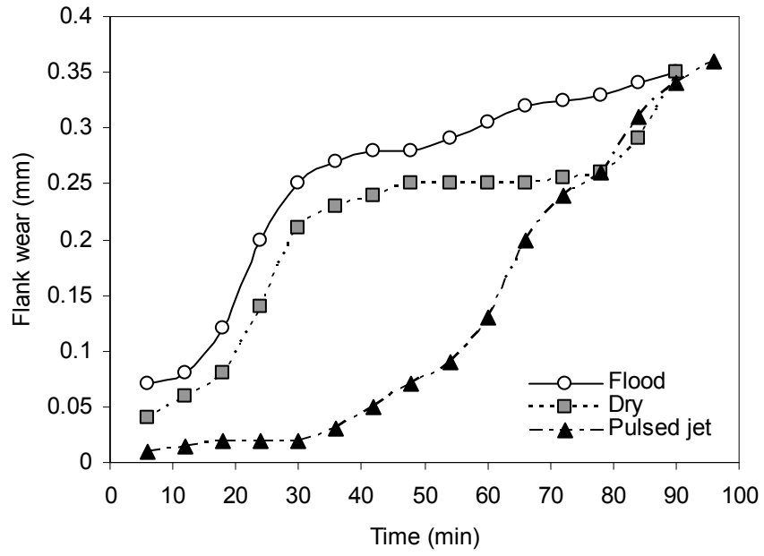
Fig. 6 Flank wear progress for slot milling
