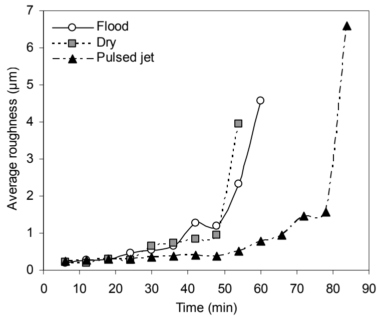
Fig. 7 Surface roughness progress for slot milling
