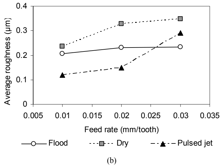
Fig. 3 Effect of feed rate on (a) flank wear and (b) surface roughness in slot milling test
